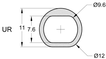
Carbon yarns Epoxy resin Pullwound tube
